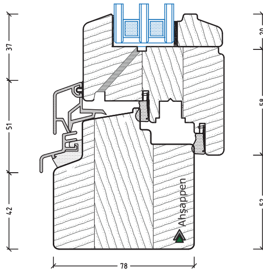
68 mm All wood detail 78 mm All wood detail 68 mm Ultraes detail
