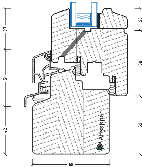
68 mm All wood detail 78 mm All wood detail 68 mm Ultraes detail
